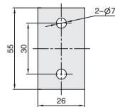
CDE-AB-30-2 方形铁片
