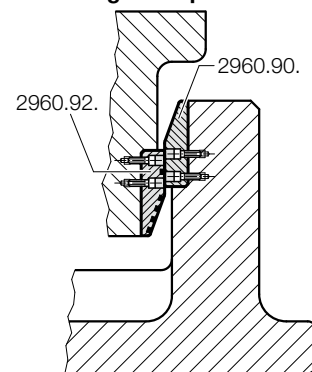
Mounting example
