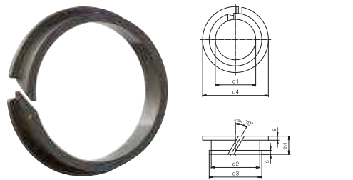
Dimensions clips bearing Abmessungen Clipslager [mm]
